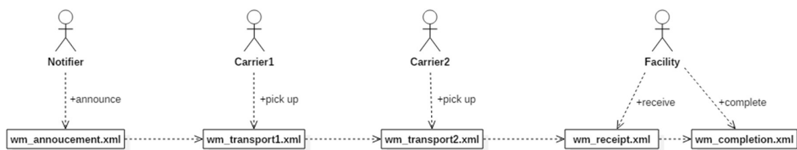
Figure 6 Movement document message creation and flow of messages
